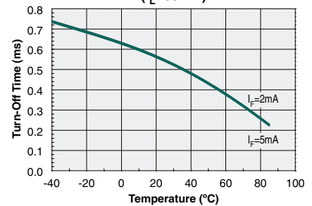
Turn-Off Time vs. Temperature ( I_L=55\text{mA} )
