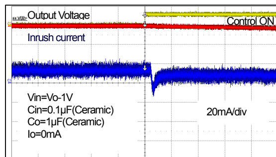
Peak current: 20mA at C_S=0.0047\mu\text{F}
