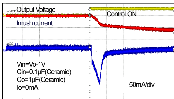
Peak current: 150mA at C_S=0\mu\text{F}
