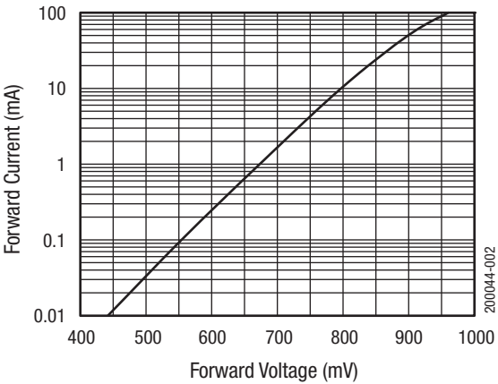
Figure 2. DC Characteristic
