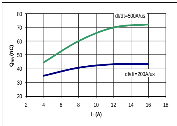
Figure 7. Typical Q_{RR} vs I_F at T_J = 125^\circ\text{C}
