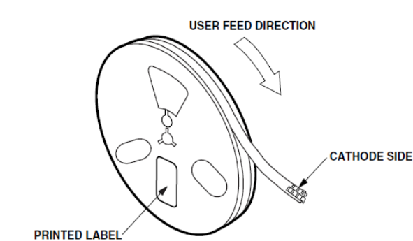
Figure 12: Reel Orientation
