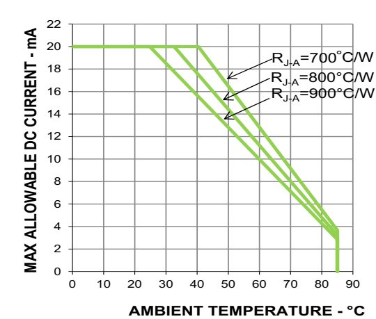
Figure 10: Derating Curve
