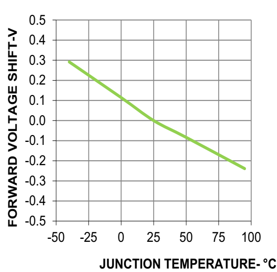
Figure 8: Forward Voltage Shift vs. Temperature
