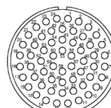
40-A60 Service A 60 Contacts, Size #16 (15)
