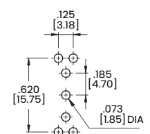
P.C.MOUNTING
