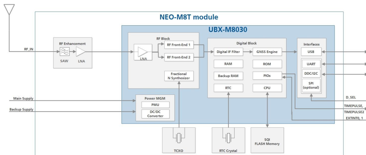
Figure 1: NEO-M8T block diagram
