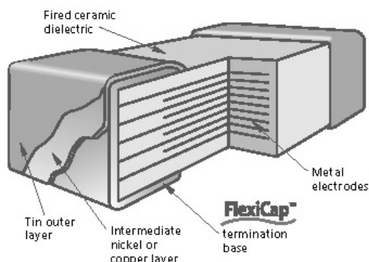
FlexiCap™ MLCC cross section
