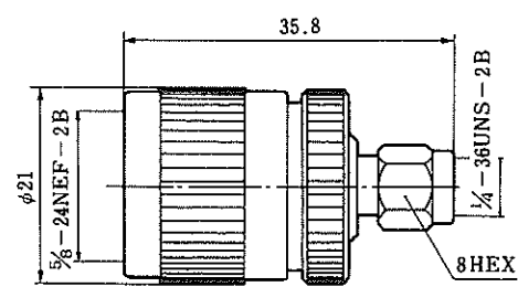
HRM-509(40)
