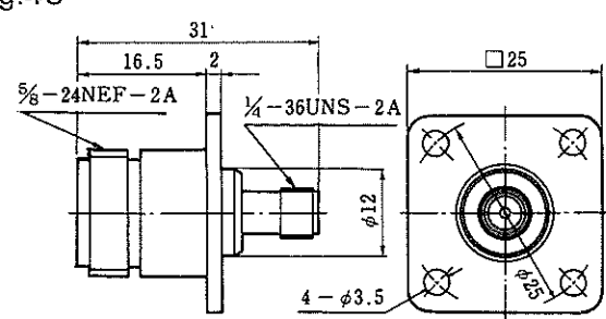
HRM-511(40) HRM-511S(40)
