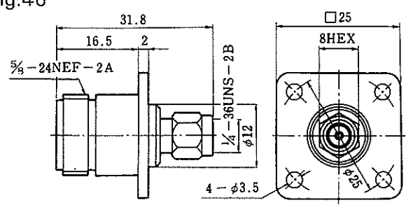
HRM-512(40) HRM-512S(40)
