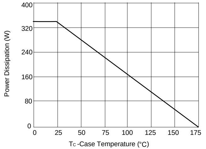
Figure 8: Power De-rating
