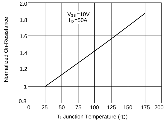
Figure 2: Rdson-Junction Temperature
