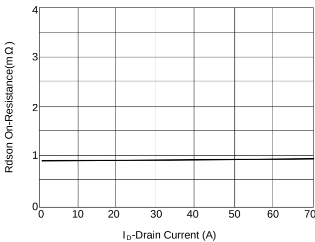
Figure 5: Rdson-Drain Current
