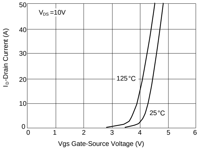
Figure 3: Transfert Characteristics
