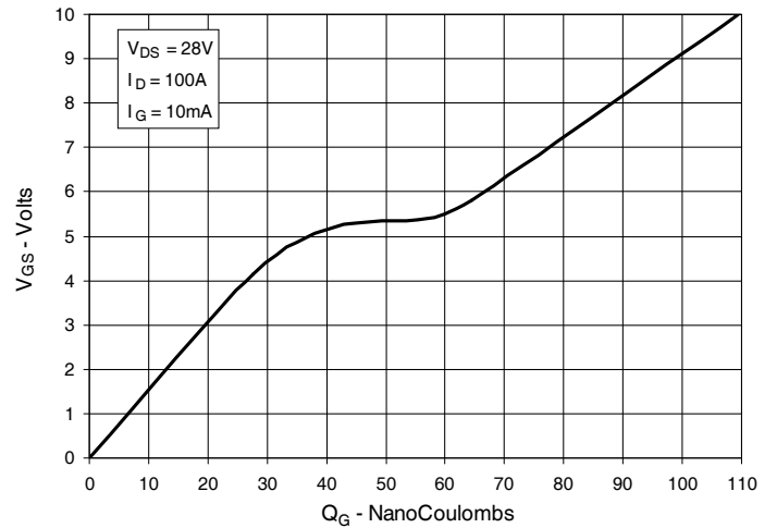
Fig. 10. Gate Charge
