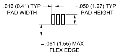
PAD DETAIL
