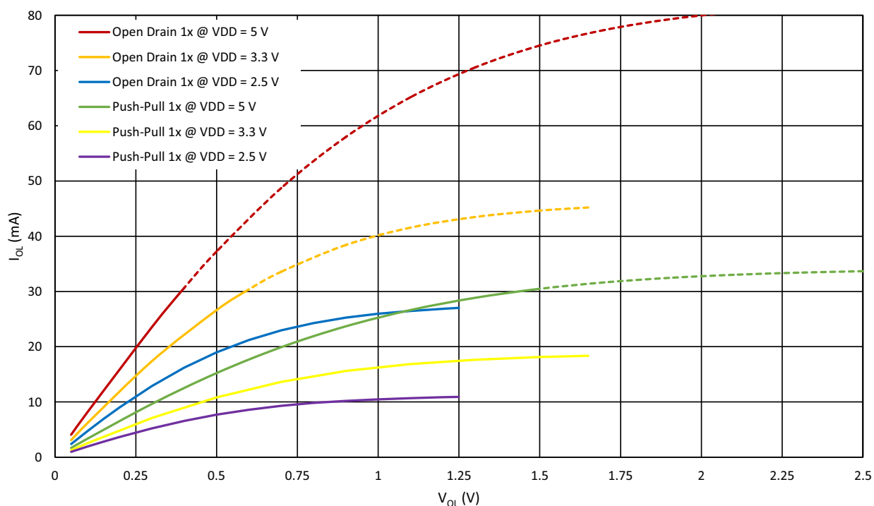
Figure 9. Typical Low Level Output Current vs. Low Level Output Voltage, 1x Drive at T_A = 25^\circ\text{C} , Full Range
