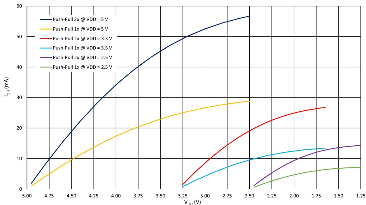
Figure 8. Typical High Level Output Current vs. High Level Output Voltage at T_A = 25^\circ\text{C}
