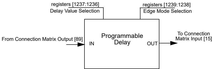
Figure 124. Programmable Delay
