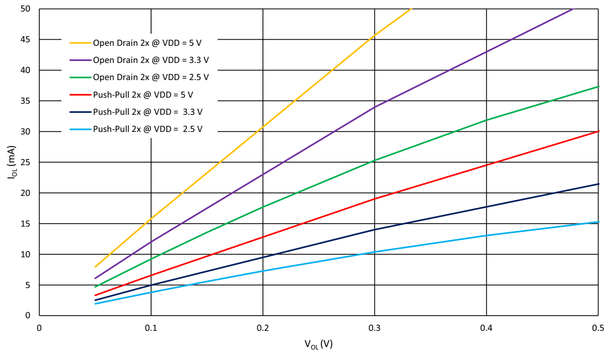
Figure 12. Typical Low Level Output Current vs. Low Level Output Voltage, 2x Drive at T_A = 25^\circ\text{C}
