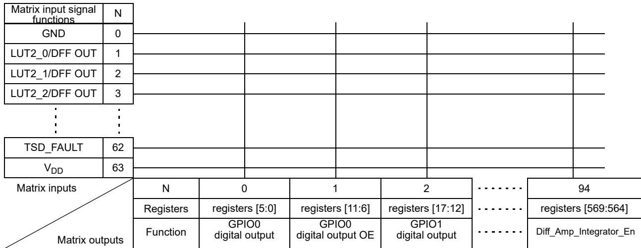
Figure 52. Connection Matrix
