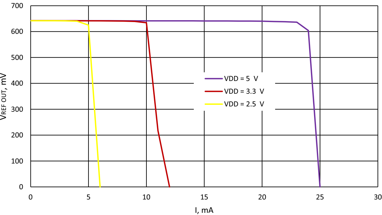
Figure 129. Typical Load Regulation, Vref = 640 mV, TA = -40 °C to +85 °C, Buffer - Enabled
