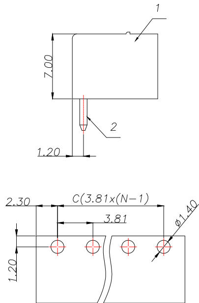
PCB LAYOUT
