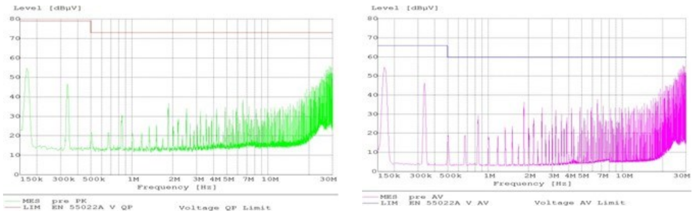
Figure 23. EMC Filter
