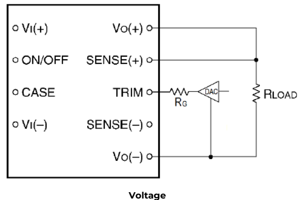
Figure 15. Circuit Configuration to Actively Adjust the Output
