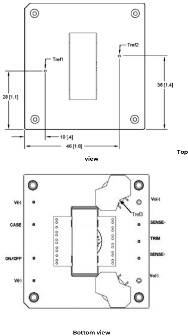
Figure 18. Case ( T_{REF} ) Temperature Measurement Location
