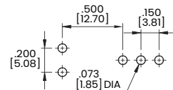
P.C.MOUNTING
