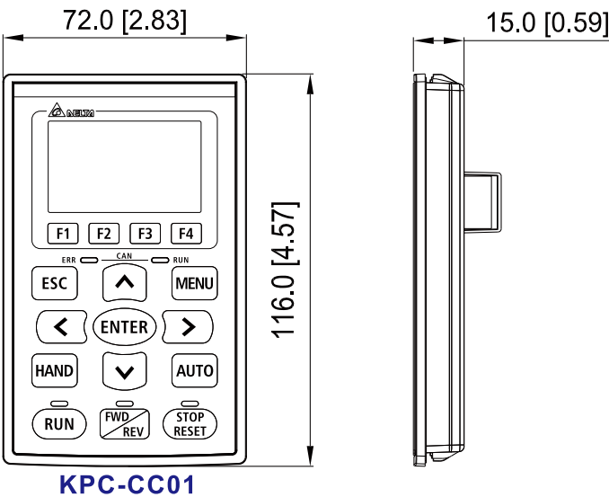
Standard LCD keypad
