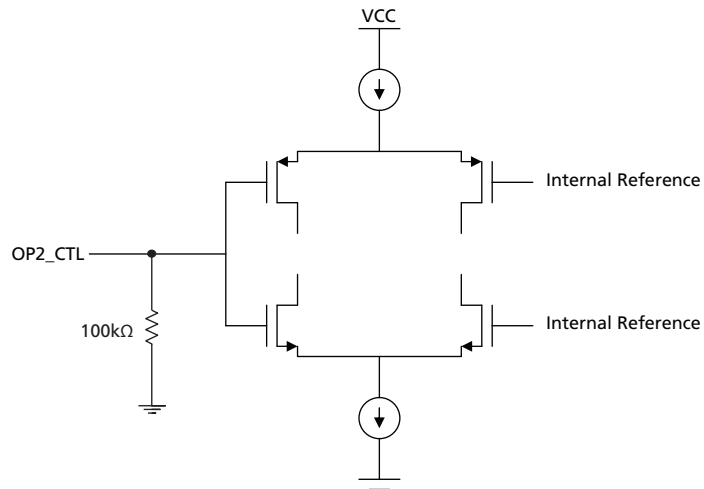
Figure 3-8: OP2_CTL
