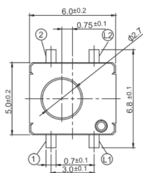
Figure 1 – 228GMV, Surface Mount Gull Wing , Vertical Actuation
