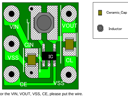
XC9235/XC9236/XC9237 A,B,C (Output Voltage Fixed) (PKG:SOT-25)
