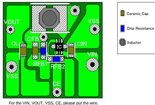
XC9235/XC9236/XC9237 D,F (Output Voltage External Setting) (PKG:USP-6C)
