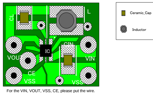
XC9235/XC9236/XC9237 A,B,C,E,G (Output Voltage Fixed) (PKG:USP-6C/USP-6EL)
