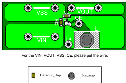
XC9235/XC9236/XC9237 A,B (Output Voltage Fixed) (PKG:WLP-5-03)
