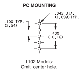
T101MH9V3BE SPDT
