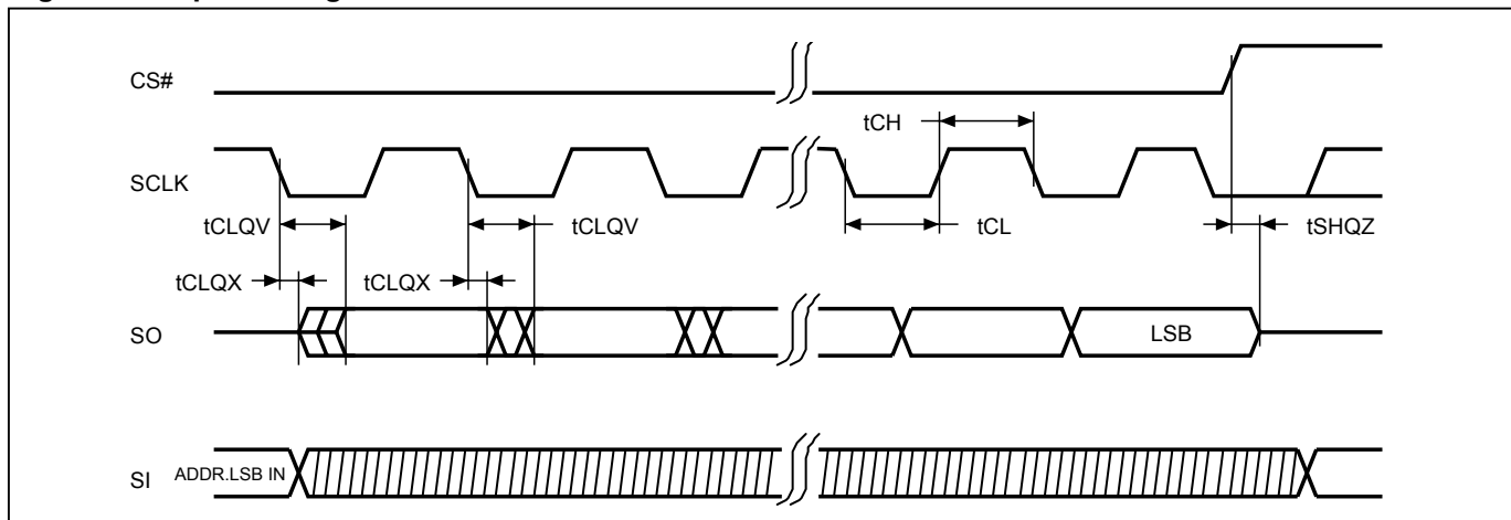
Figure 3. Output Timing
