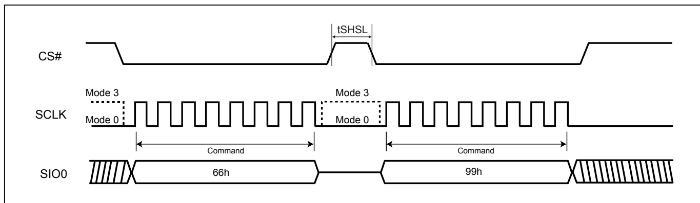
Figure 27. Reset Sequence
