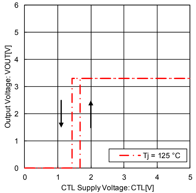
Figure 20. CTL ON / OFF Mode Voltage ( T_j = 125^{\circ}\text{C} )
