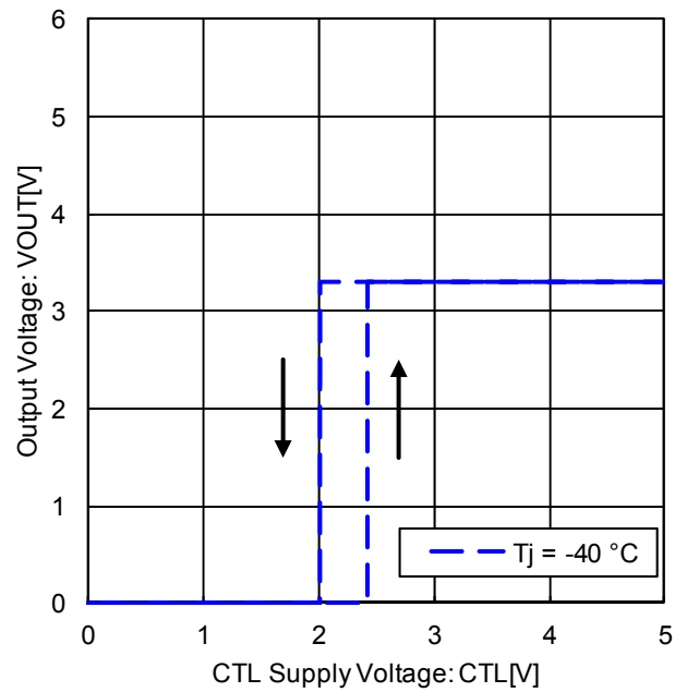
Figure 18. CTL ON / OFF Mode Voltage ( T_j = -40^{\circ}\text{C} )
