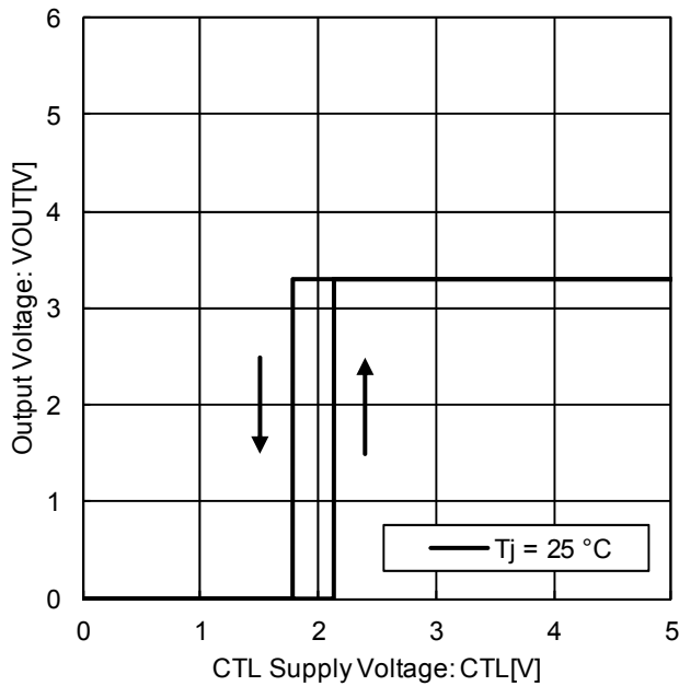
Figure 19. CTL ON / OFF Mode Voltage ( T_j = 25^{\circ}\text{C} )
