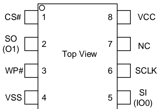
8 - LEAD VSOP/SOP/DIP
