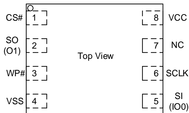
8 - LEAD USON
