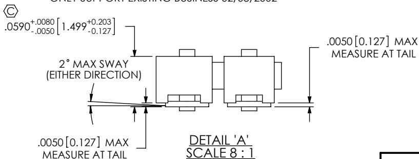
FIG 4 -MW: METAL WASHER OPTION MTMM-1XX-02-XX-X-100-MW SHOWN (ONE PER POSITION) (-D & Q PODY SPEC ONLY, SEE NOTE 5) (SAME AS FIG 1, DIFFERENT AS SHOWN) ** -MW OPTION, DO NOT DESIGN IN. SAMTEC WILL ONLY SUPPORT EXISTING BUSINESS 02/08/2002
