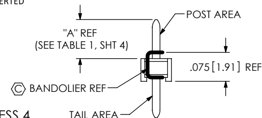
IN PROCESS 4 (-T PLATING ONLY) (SEE NOTE 6 & TABLE 3)
