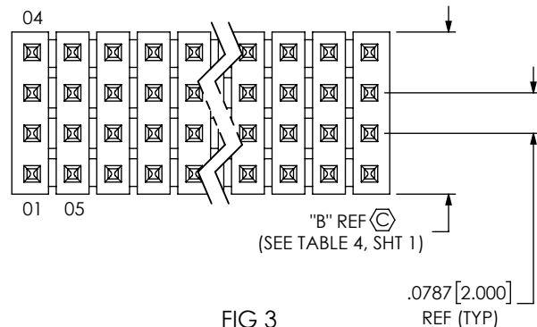
FIG 3 -Q: QUAD ROW OPTION MTMM-1XX-02-XX-Q-100 SHOWN (SAME AS FIG 1, DIFFERENT AS SHOWN)
