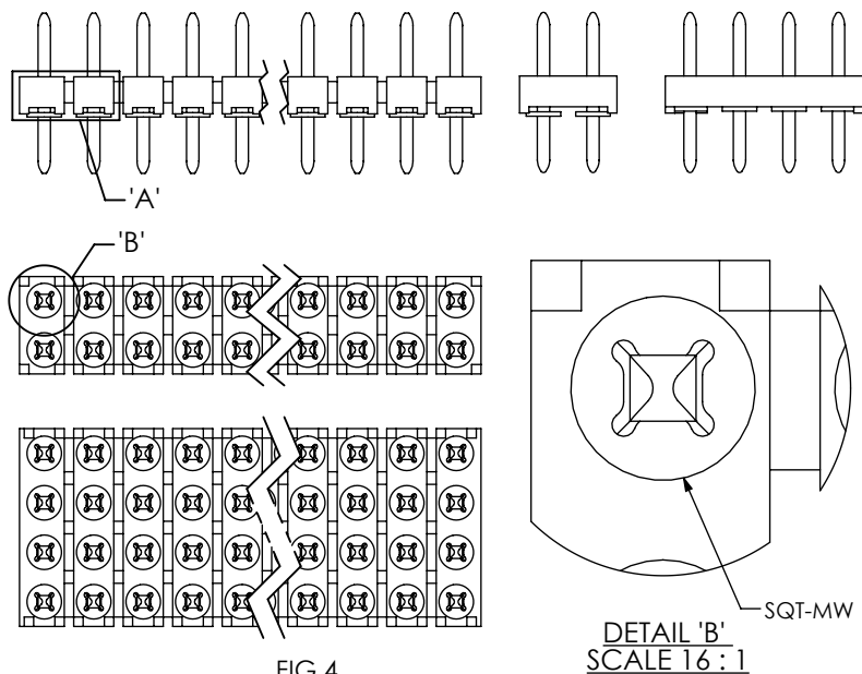
FIG 4 -MW: METAL WASHER OPTION MTMM-1XX-02-XX-X-100-MW SHOWN (ONE PER POSITION) (-D & Q PODY SPEC ONLY, SEE NOTE 5) (SAME AS FIG 1, DIFFERENT AS SHOWN) ** -MW OPTION, DO NOT DESIGN IN. SAMTEC WILL ONLY SUPPORT EXISTING BUSINESS 02/08/2002
