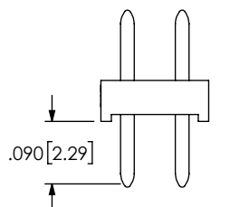
IN PROCESS 1 SCALE 4:1
