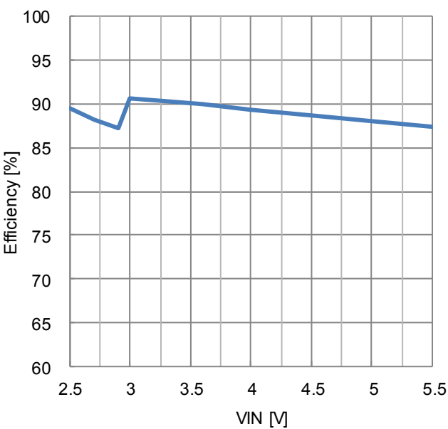
Figure 16. Efficiency vs VIN PWM/PFM Auto mode, Iout=125mA L : DFE252012C1R0
