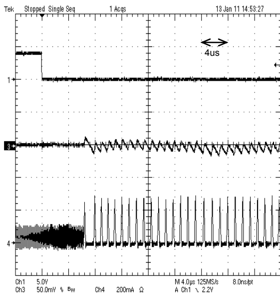
Figure 12. Mode Change Response MODE : High to Low
