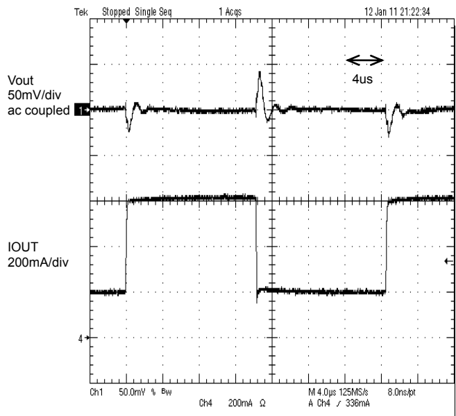
Figure 9. Load transient response 200mA to 600mA t_r=t_f=100\text{ns} , MODE : Low
