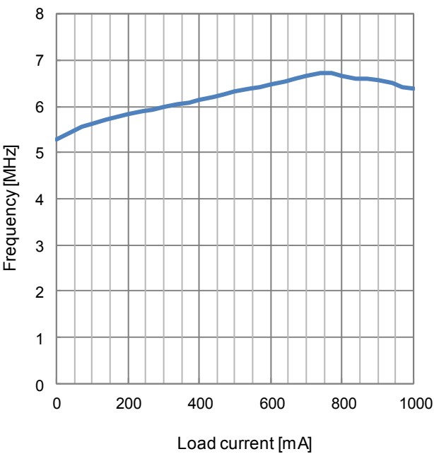
Figure 18. Frequency vs Load current PWM mode Operation
