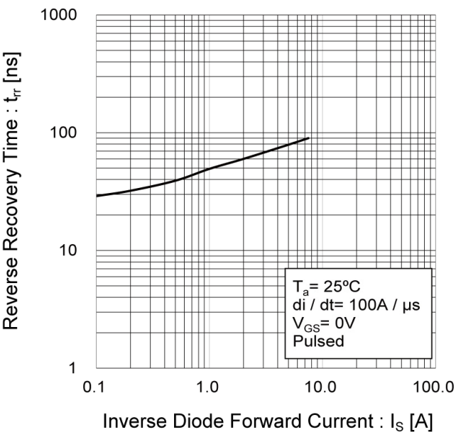
Fig.21 Source Current vs. Reverse Recovery Time
