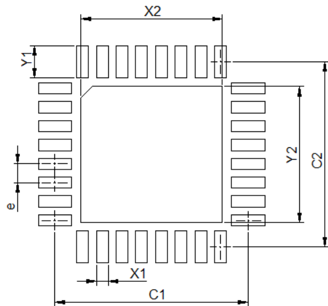
Figure 6.2. 32-Pin, QFN Land Pattern
