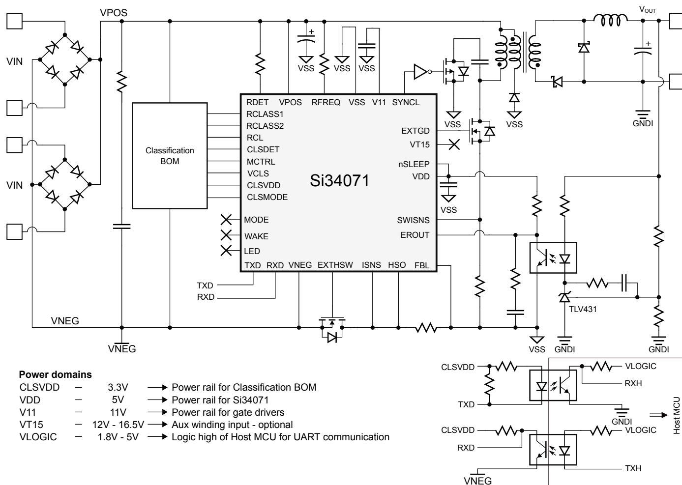
Figure 3.1. Si34071 Simplified Isolated Forward Application Diagram
