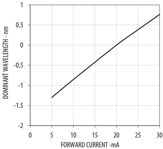
Figure 6: Wavelength Shift vs. Forward Current
