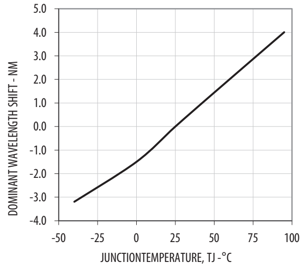
Figure 9: Wavelength Shift vs. Temperature
