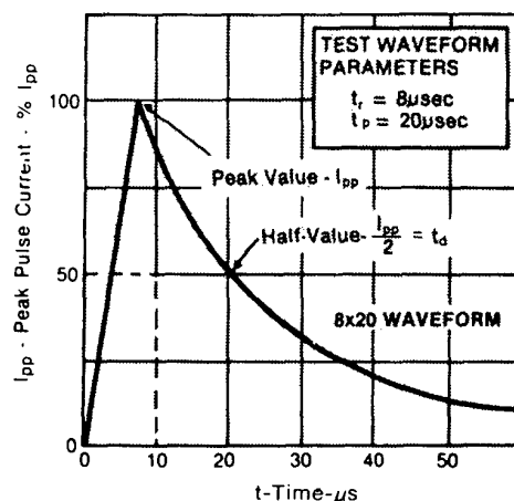
FIGURE 2 Pulse Waveform
