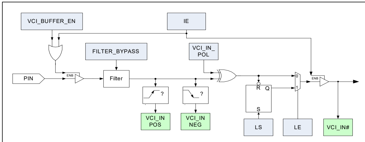
FIGURE 42-3: VBAT-POWERED CONTROL INTERFACE BLOCK DIAGRAM
