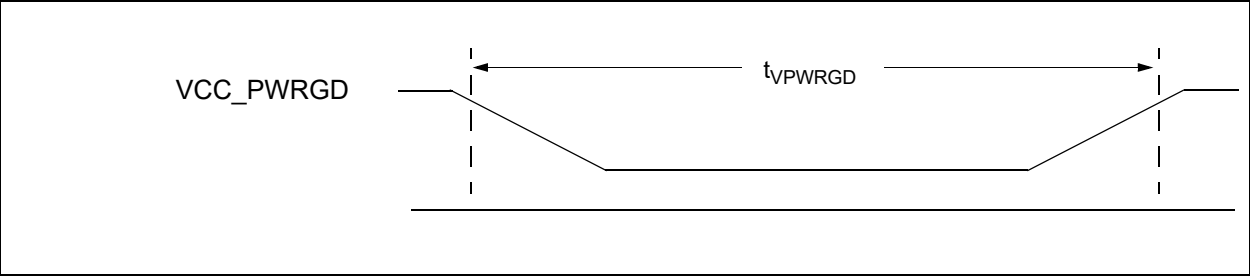
FIGURE 50-7: VCC_PWRGD TIMING
