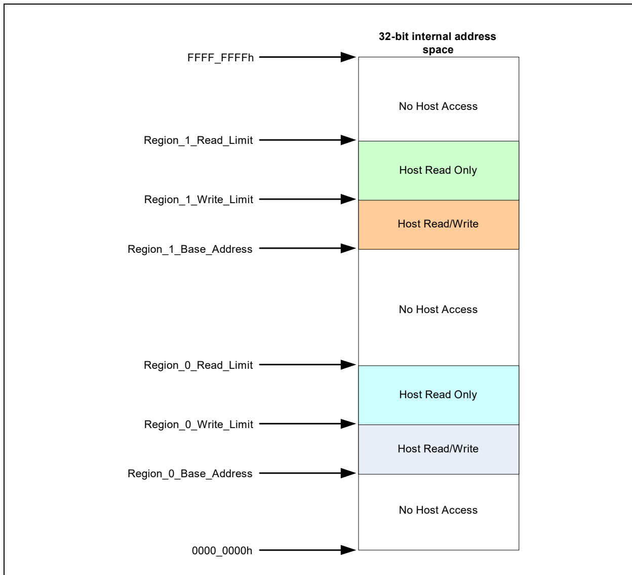
FIGURE 14-3: EMBEDDED MEMORY ADDRESSING
