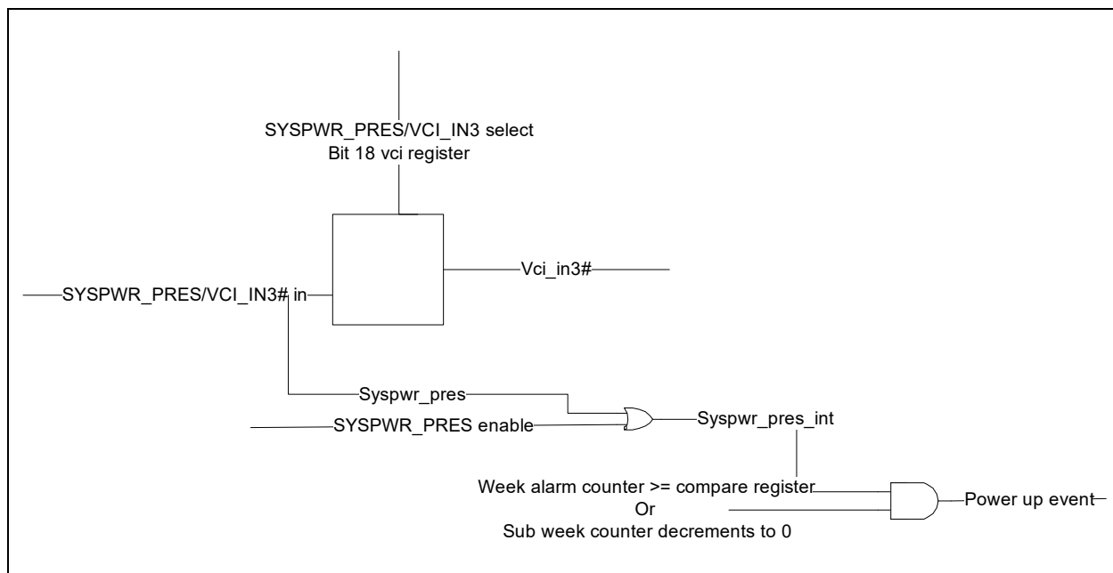
FIGURE 24-2: SYSPWR_PRES SELECT
