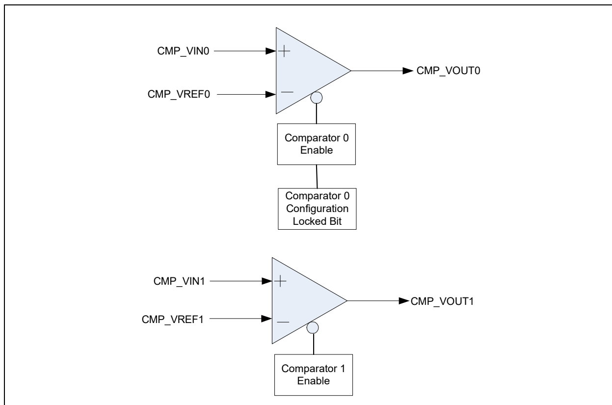
FIGURE 30-2: COMPARATOR BLOCK DIAGRAM
