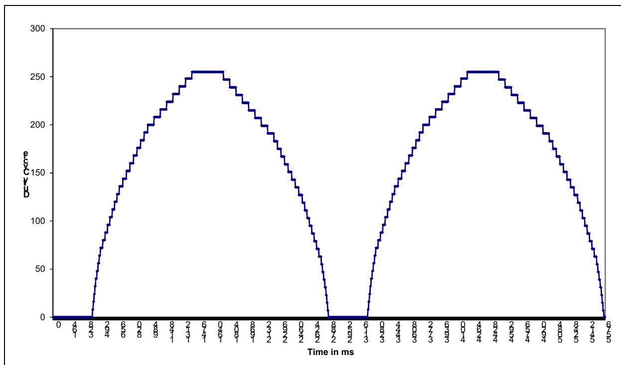
FIGURE 31-6: NON-LINEAR BRIGHTNESS CURVE EXAMPLE
