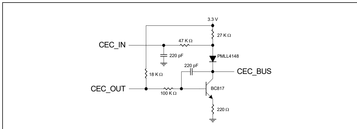
FIGURE 28-2: CEC BUS APPLICATION EXAMPLE
