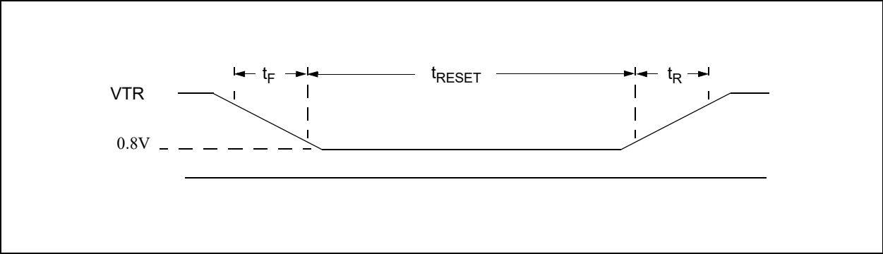
FIGURE 50-4: NRESET_IN TIMING
