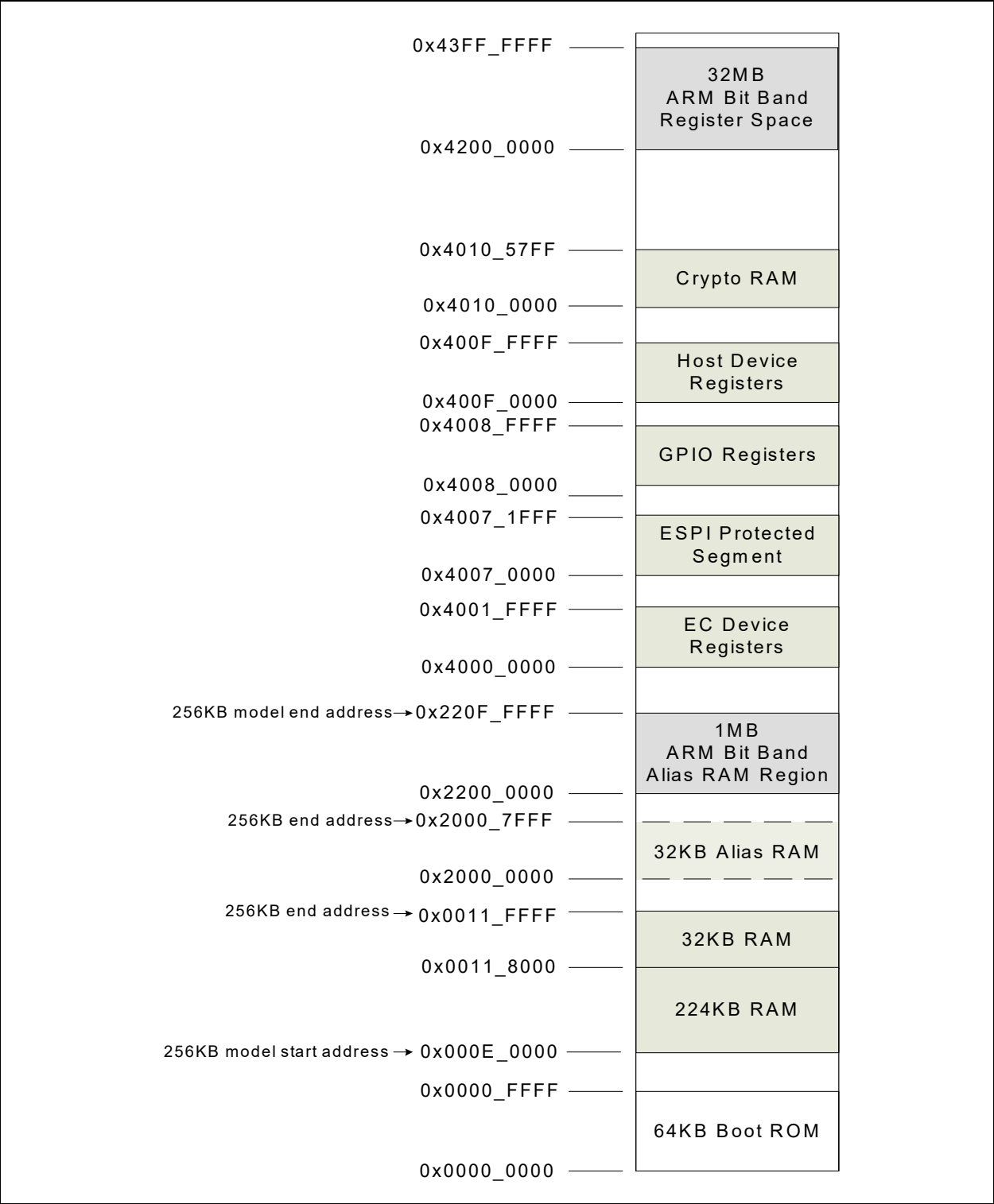
FIGURE 6-1: MEMORY LAYOUT
