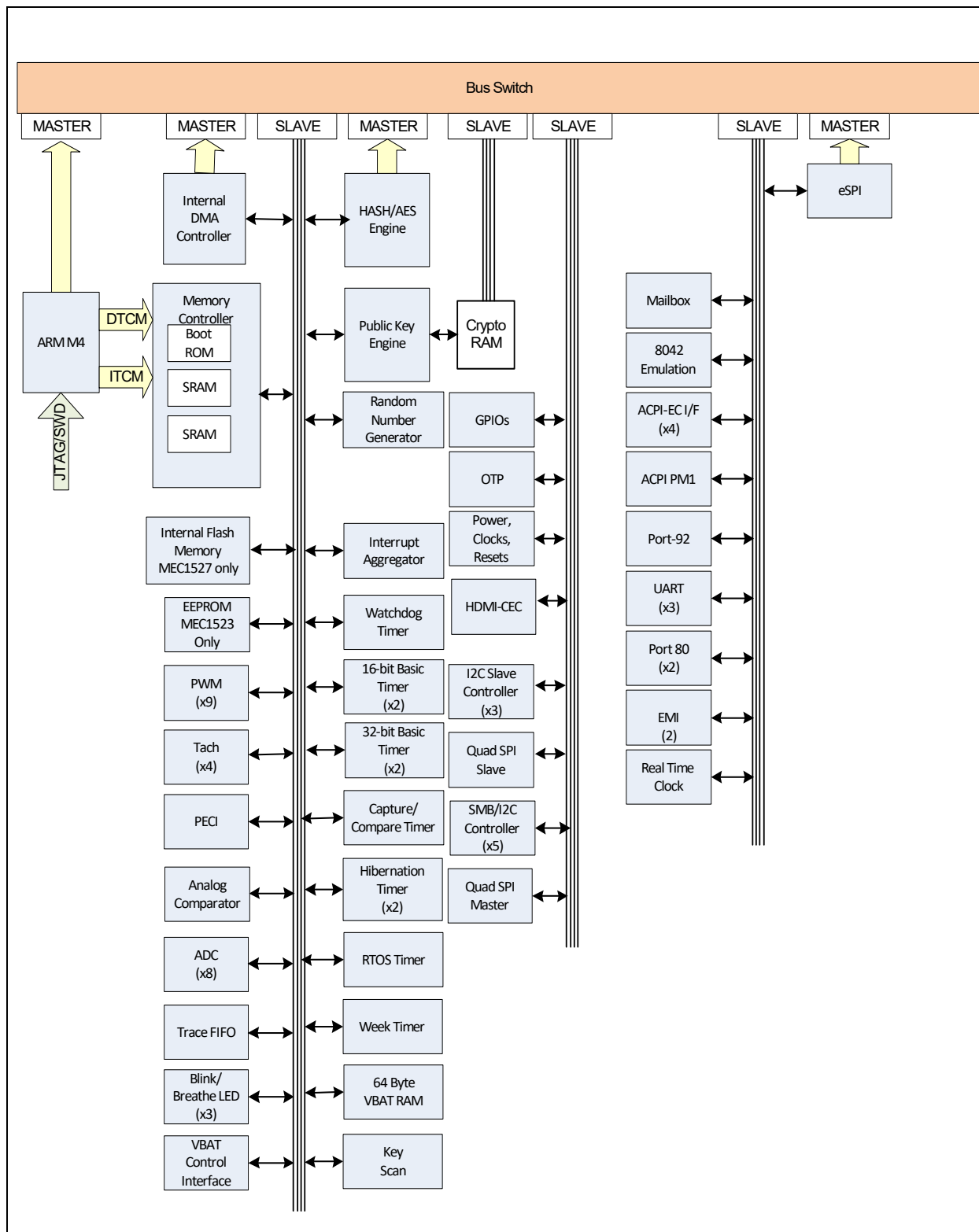
FIGURE 1-1: BLOCK DIAGRAM
