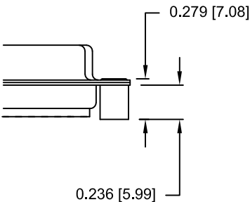
02X ..... 0.236" (SOLDER SIDE)
