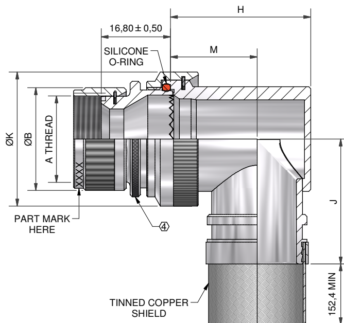
90° BACKSHELL - TYPE 2
