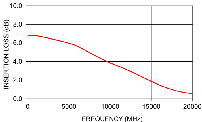
EQY-6-24+ INSERTION LOSS
