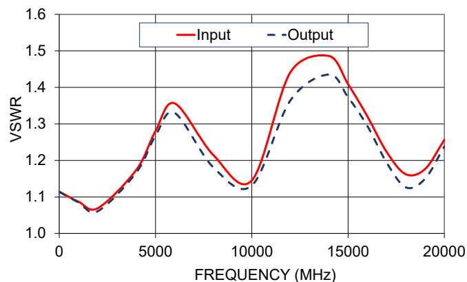
EQY-6-24+ VSWR
