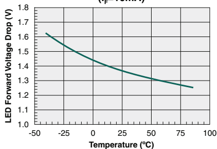
Typical LED Forward Voltage Drop vs. Temperature ( I_F=10\text{mA} )
