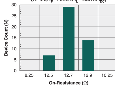
Typical On-Resistance Distribution (N=50, I_F=10\text{mA} , I_L=120\text{mA}_{DC} )
