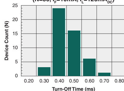
Typical Turn-Off Time (N=50, I_F=10\text{mA} , I_L=120\text{mA}_{DC} )
