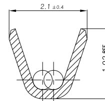
SECTION "B-B" Scale 20/1
