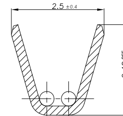
SECTION "A-A" Scale 20/1
