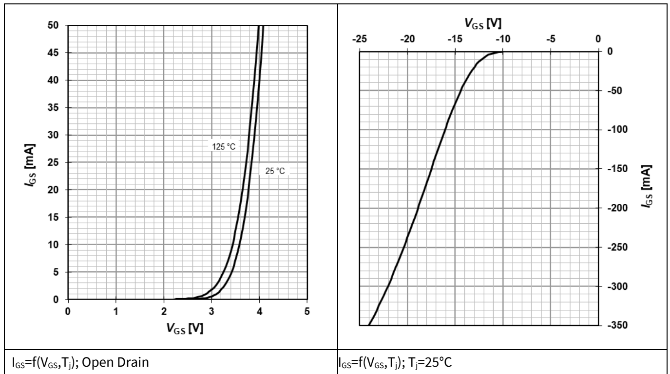
Figure 11 Typical gate characteristics forward and reverse
