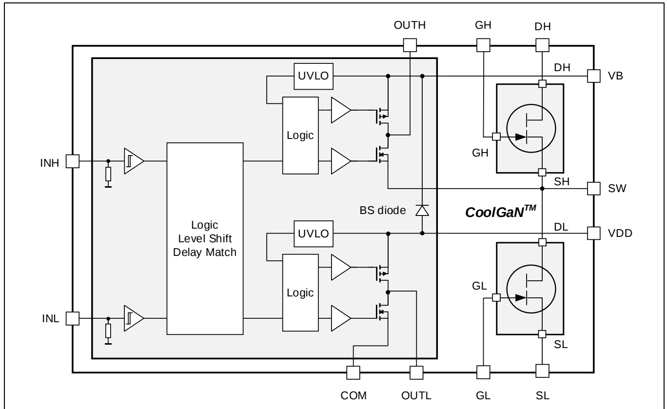
Figure 3 Block Diagram IGI60L5050A1M
