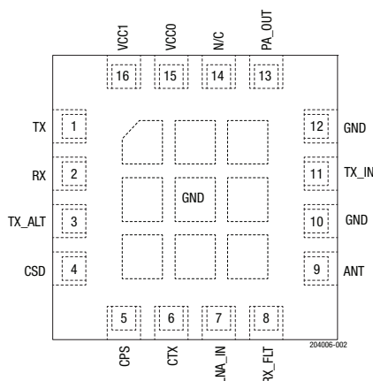
Figure 2. SKY66420-11 Pinout (Top View)
