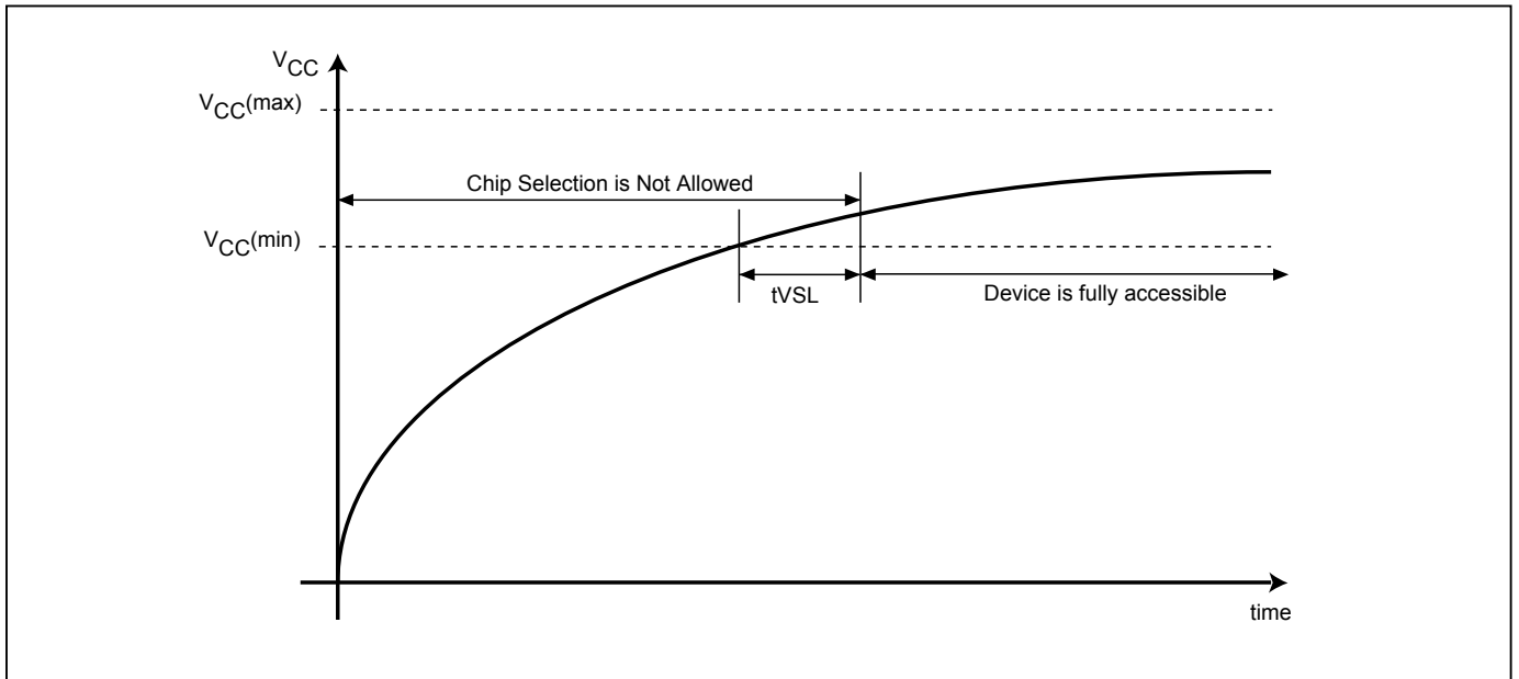
Figure 29. Power-up Timing
