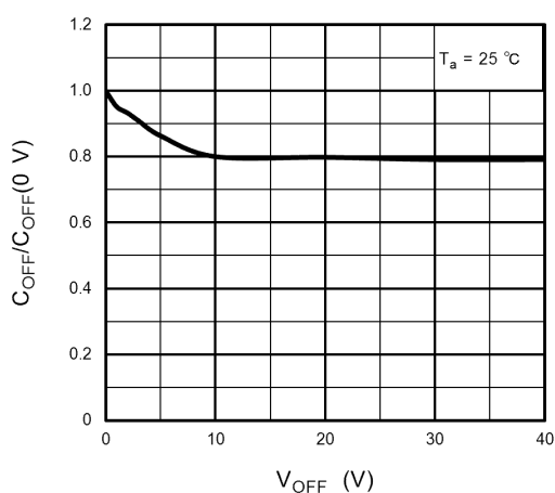
Fig. 12.1.11 C_{OFF}/C_{OFF}(0V) - V_{OFF}
