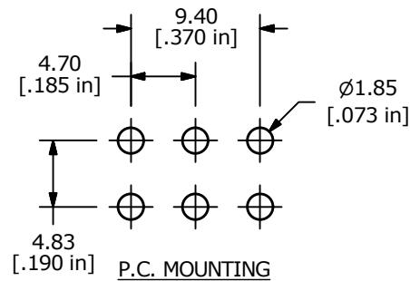
P.C. MOUNTING
