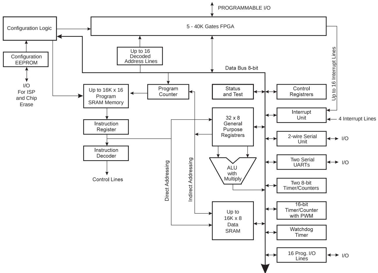
Figure 1. AT94S Architecture
