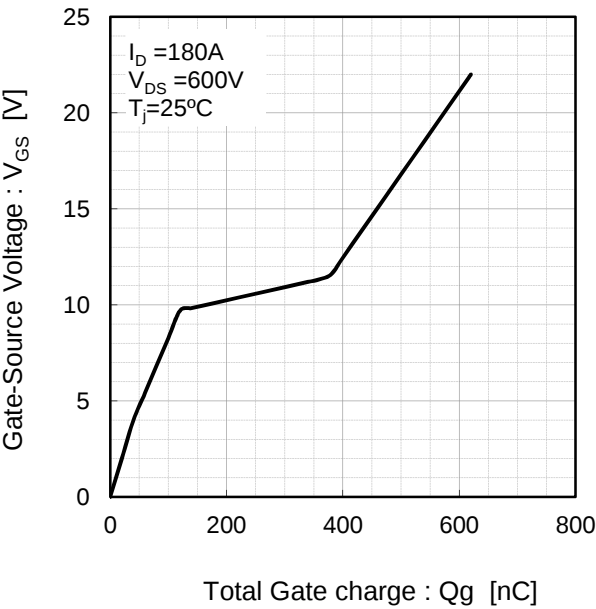
Fig.25 Gate Charge Characteristics
