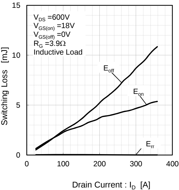
Fig.14 Switching Loss vs. Drain Current [ T_J=150^{\circ}\text{C} ]
