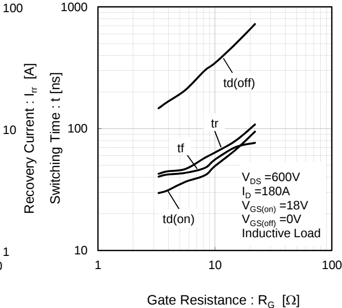
Fig.18 Switching Characteristics vs. Gate Resistance [ T_j=25^{\circ}\text{C} ]
