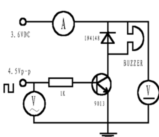
Test Circuit
