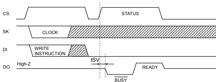
Figure 44 R/\bar{B} Status Output Timing Chart
