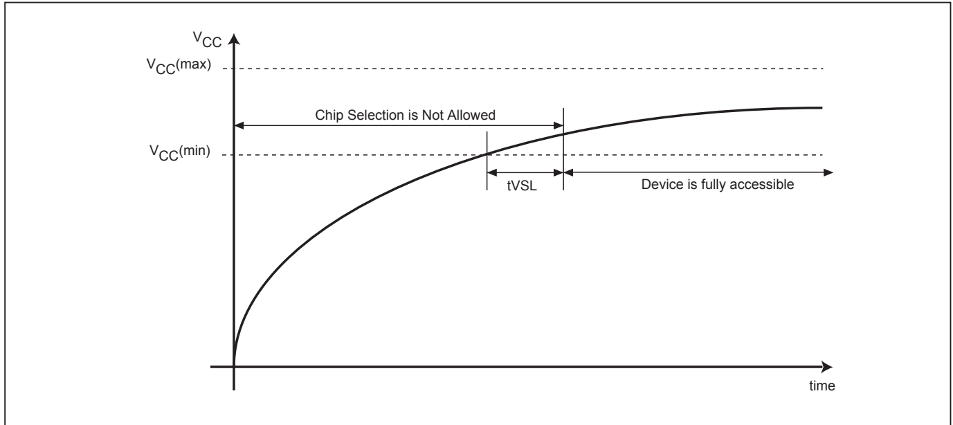
Figure 39. Power-up Timing
