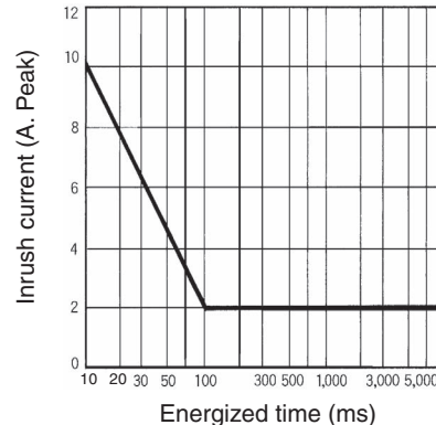
G3FD-102SN-VD/102S-VD
