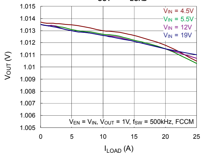
V_{OUT} vs. I_{LOAD}
