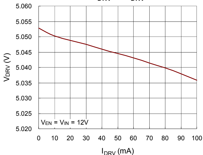
V_{DRV} vs. I_{DRV}
