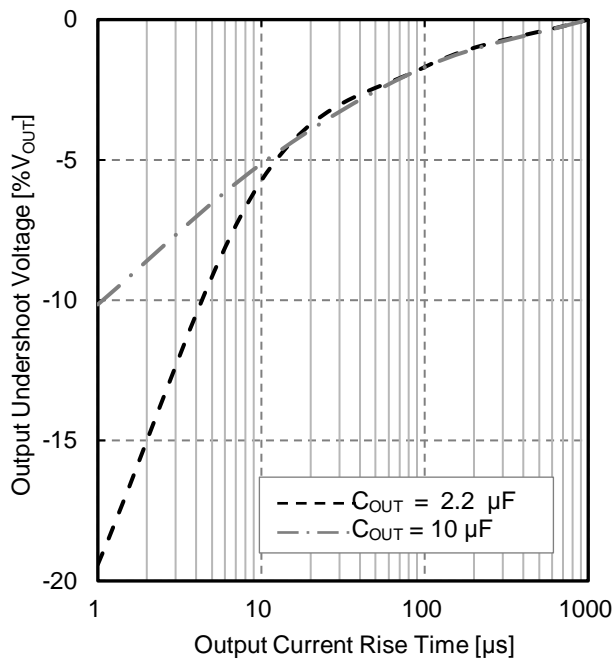
(e. I_{OUT} = 10\text{ mA} \rightarrow 700\text{ mA} , C_{ADJ} = \text{None} )
